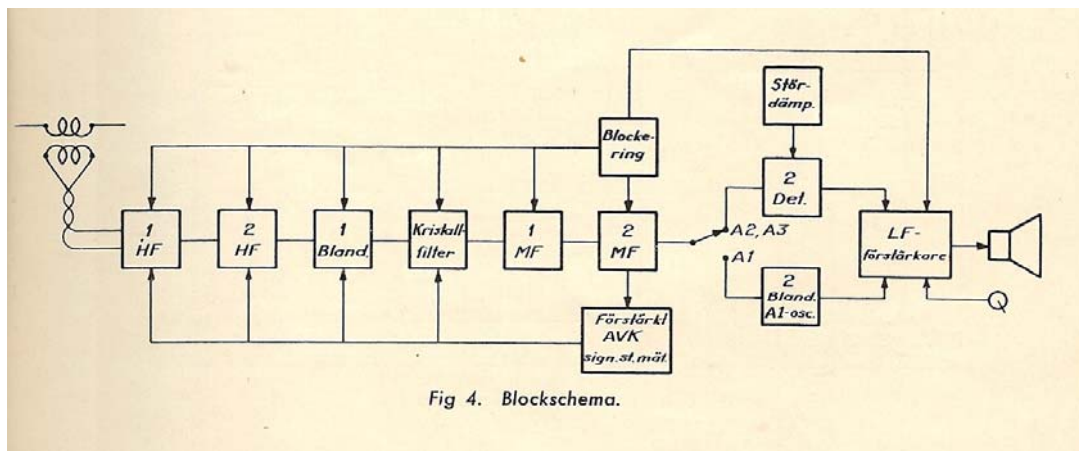
Mrm 6 blockschema.
