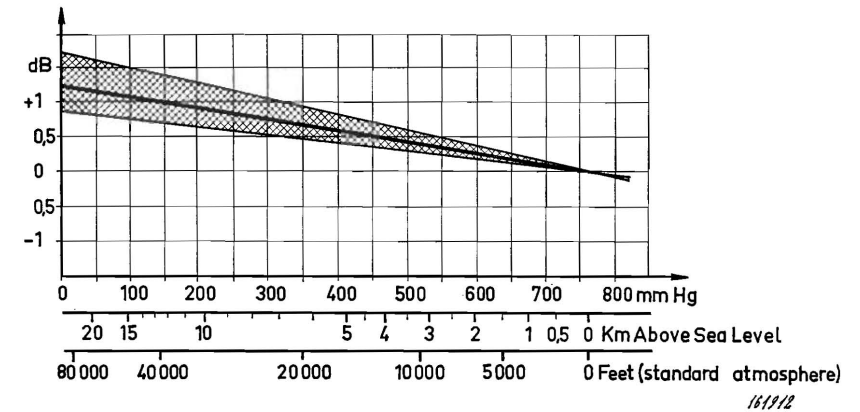
Fig. 5.2. Microphone sensitivity at 400 Hz as a function of the static ambient pressure. The corresponding altitudes are also given on the curve.
