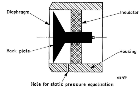
Fig. 2.3. Schematic construction of a condenser microphone cartridge.
