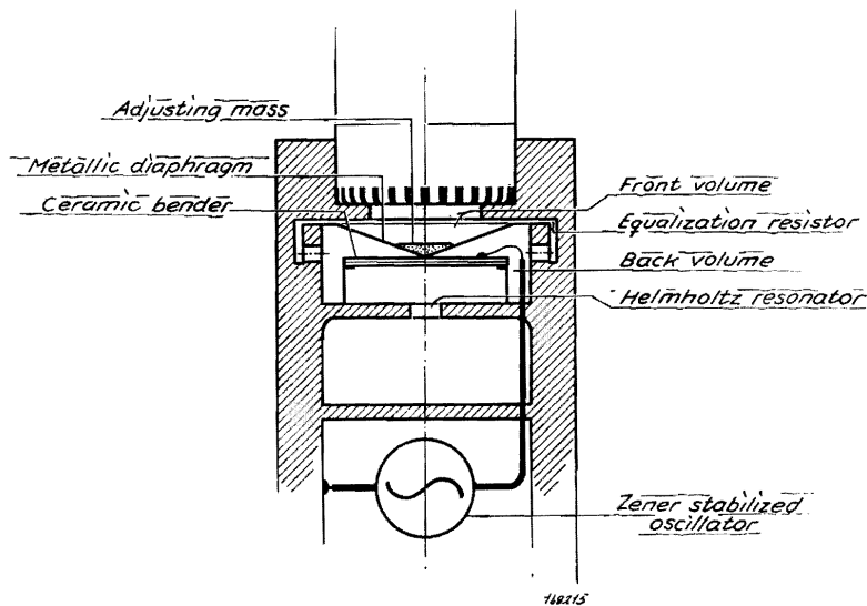
Fig. 7.5. Schematic of the Calibrator Type 4230.
