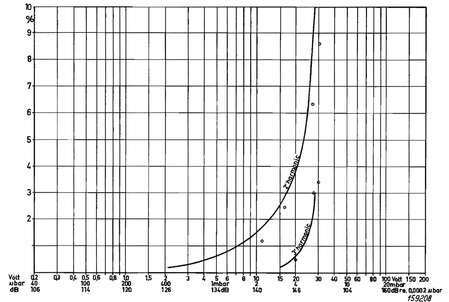
Fig. 5.9. Typical distortion curves for the one-inch microphones. The curves in full are measured on the source-follower and referred to a complete microphone with a sensitivity of 5 \text{ mV}/\mu\text{bar} . The measuring points shown are averages measured in a pistonphone on a number of complete microphones at 50 Hz.
