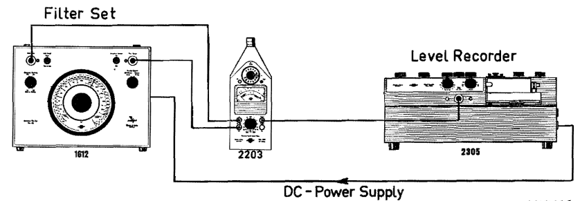
Fig. 9.9. Set-up for the recording of noise spectrograms.
