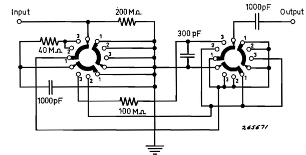
Fig. 4.3. Circuit diagram for the Integrator ZR 0020.
