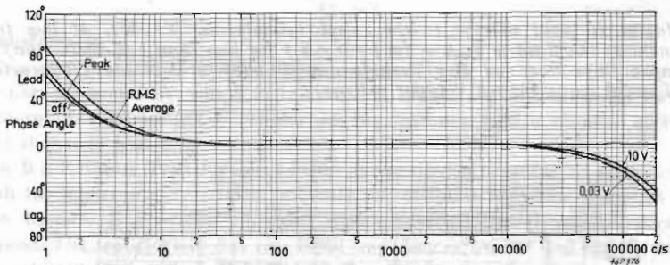
Fig. 14. Typical phase-frequency response for the Electronic Voltmeter Type 2409/2416. At low frequencies the phase shift is somewhat dependent upon the METER SWITCH setting, and at high frequencies, upon METER RANGE.
