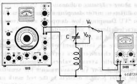
Fig. 9. Measurement of quality-factor of inductances.
