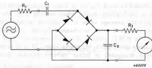
Fig. 18. The circuit used to obtain Peak indication.
