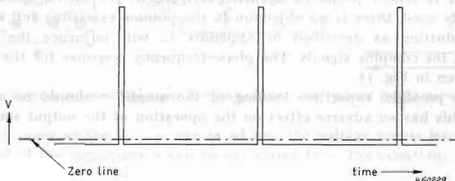
Fig. 5. Example of unsymmetrical signal with a crest factor of approximately 5.
