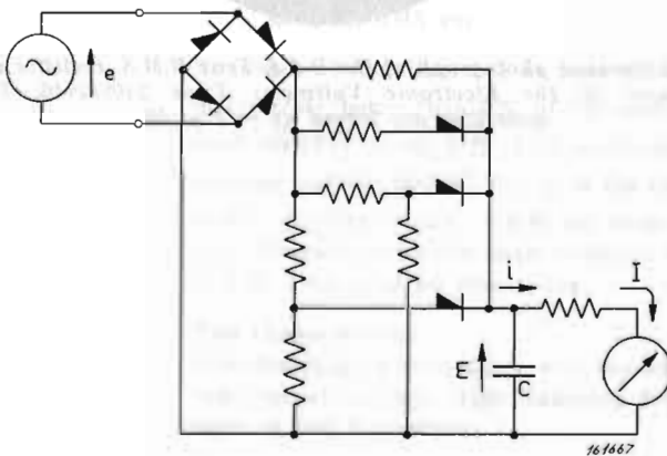
Fig. 20. Schematic diagram of the R.M.S. rectifier circuit having characteristics of the type shown in Fig. 21.
