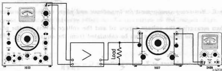
Fig. 8. Measuring arrangement for distortion measurements.
