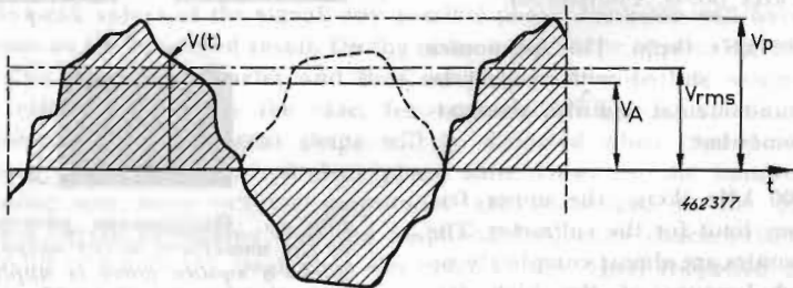
Fig. 16. Example of a periodic signal with indication of the Peak, R.M.S., and Average values of the voltage.
