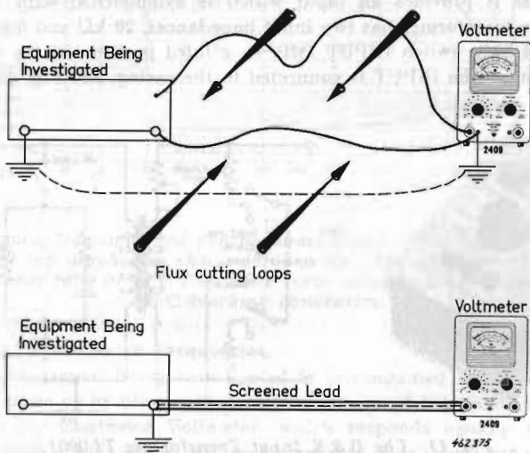
Fig. 10. When measuring small signals, use screened leads (bottom picture) and try to avoid ground loops. An arrangement such as that in the top picture is inherently un-sound but is particularly bad practice when using a high impedance instrument like the 2409/2416.
