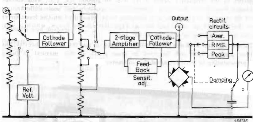
Fig. 2. Block diagram of Type 2409.
