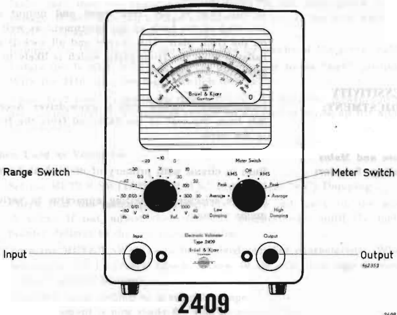
Fig. 4. Front View of the Electronic Voltmeter Type 2409.
