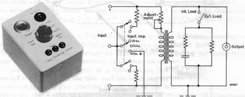
Fig. 11. The B & K Input Transformer TI 0001.
