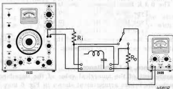
Fig. 7. Measurement of amplification and frequency response of amplifiers, filters etc.
