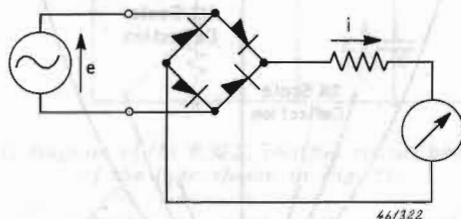
Fig. 17. Schematic diagram of Average rectifier.
