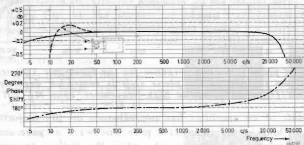
Fig. 13. Typical frequency and phase characteristics of the Input Transformer T10001. The top graph also shows (broken line) the tolerance of \pm 2\% on the transformer ratio of 1 : 1. The phase curve refers to a direct input with no D.C.-blocking condensers.
