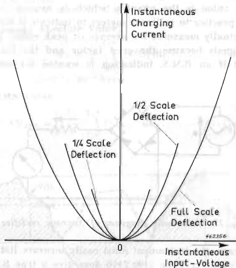
Fig. 19. Ideal R.M.S. rectifier characteristics.
