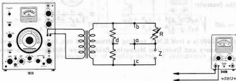
Fig. 6. Measuring arrangement for impedance and phase angle measurements.
