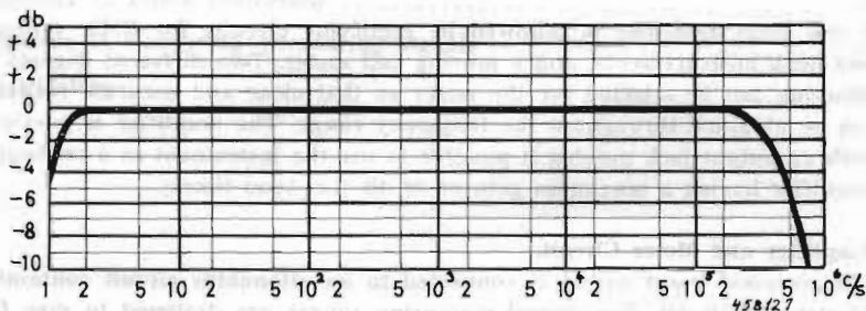
Fig. 3. Typical frequency response of the Electronic Voltmeter Type 2409.
