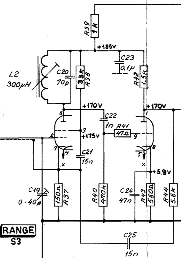
V4 E80CF Preamplifier
