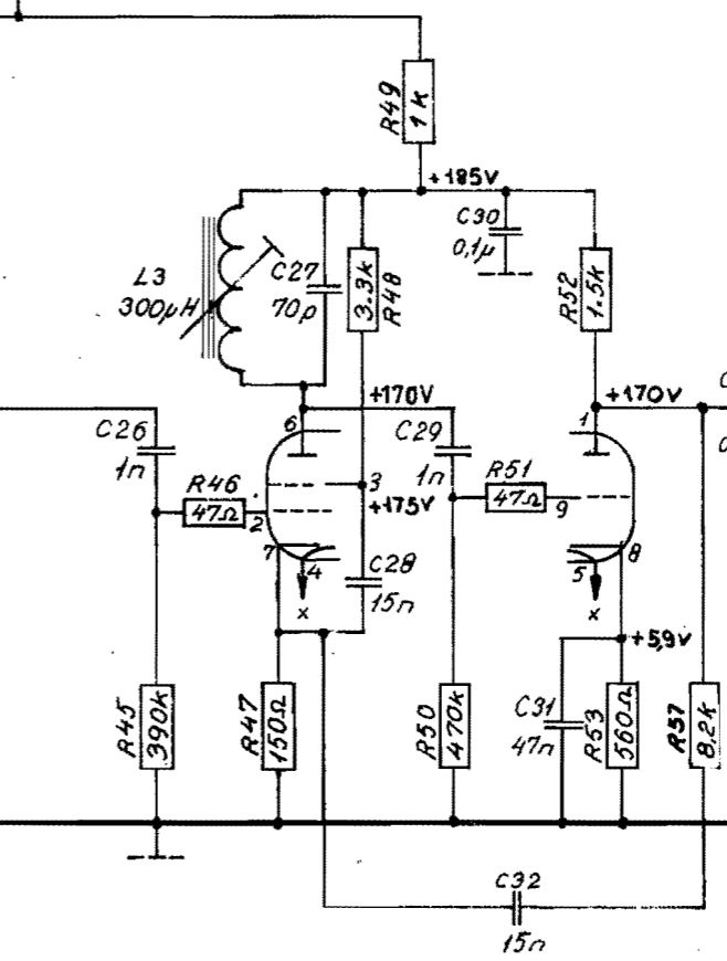
V5 E80CF Amplifier
