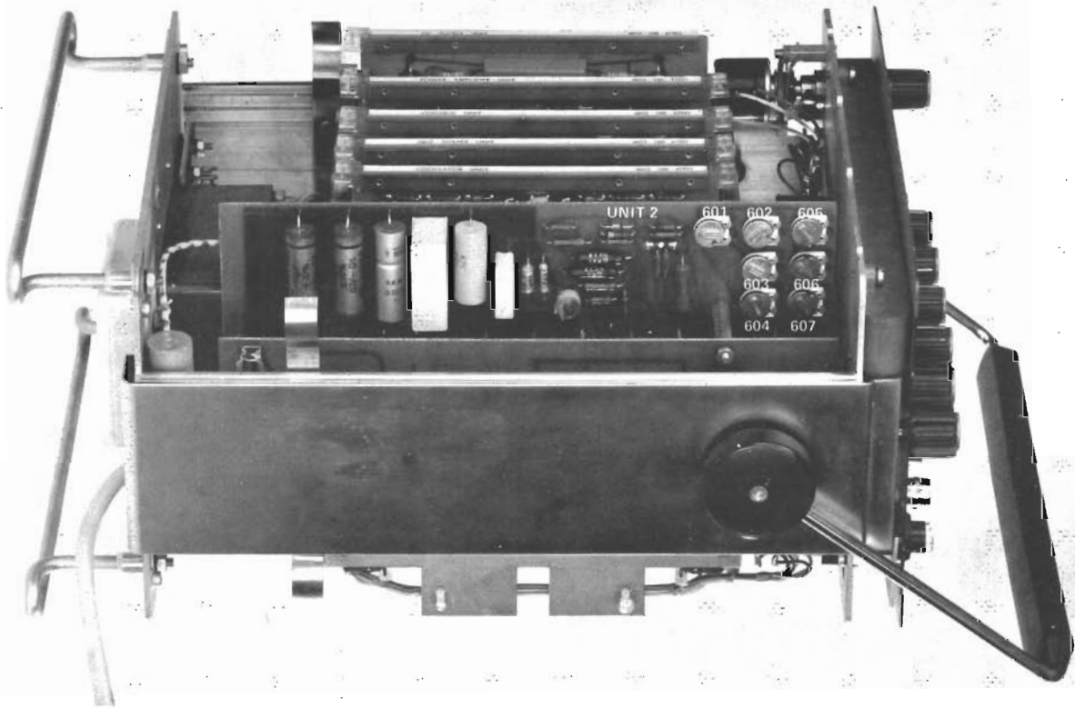
Fig. 10. Adjusting elements on UNIT 2
