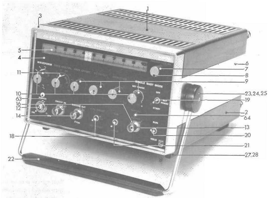
Fig. 12. Front view, mechanical components
