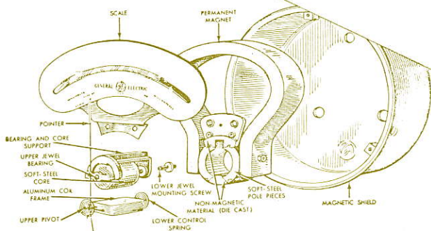
Fig. 2-1(b) Disassembled parts of a typical permanent-magnet moving coil instrument.
