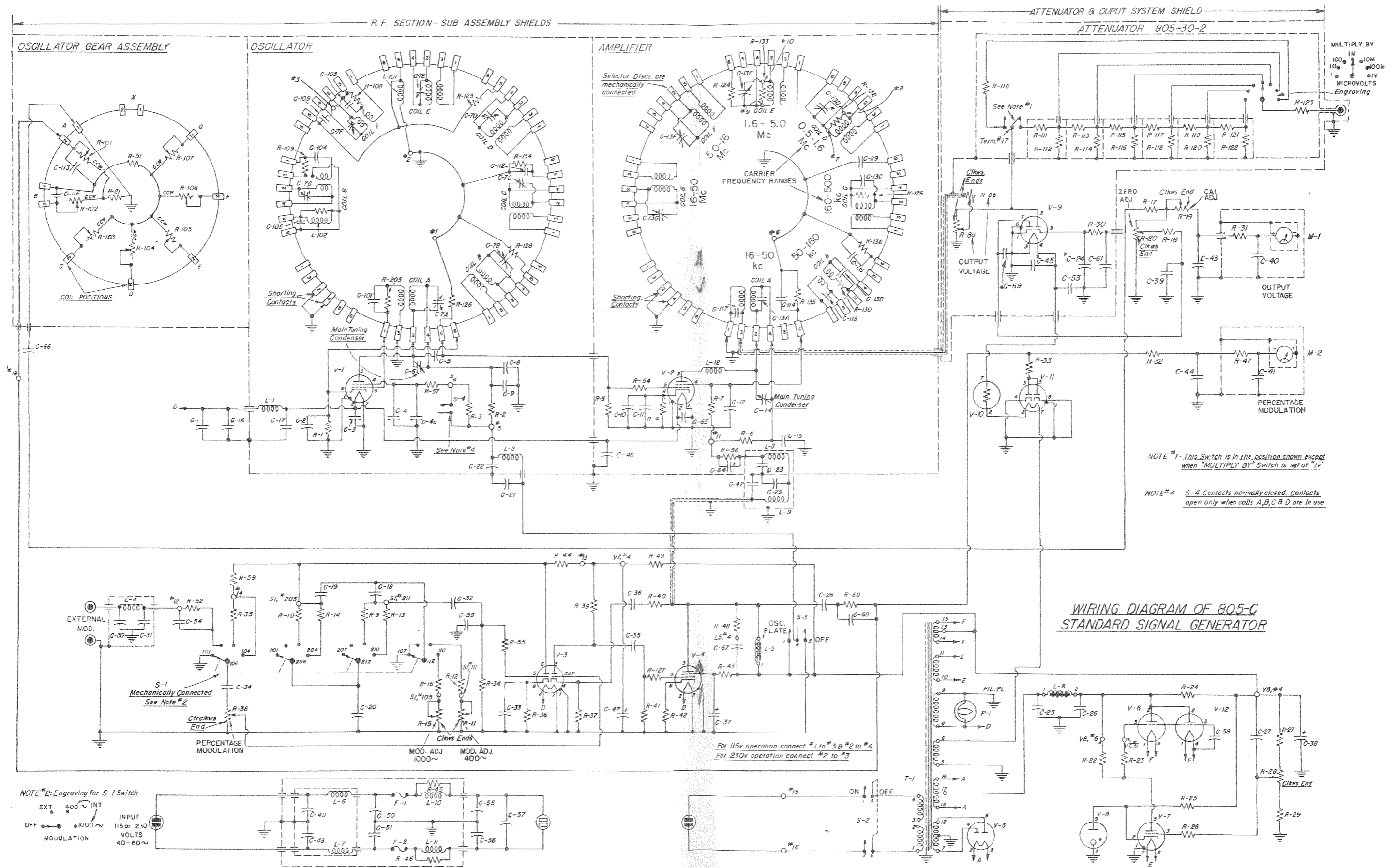
FIGURE 2. WIRING DIAGRAM FOR TYPE 805-C STANDARD-SIGNAL GENERATOR.
