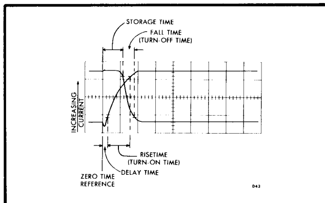
Fig. 2-4. Double-triggered display of the switching characteristics of a p-n-p transistor.
