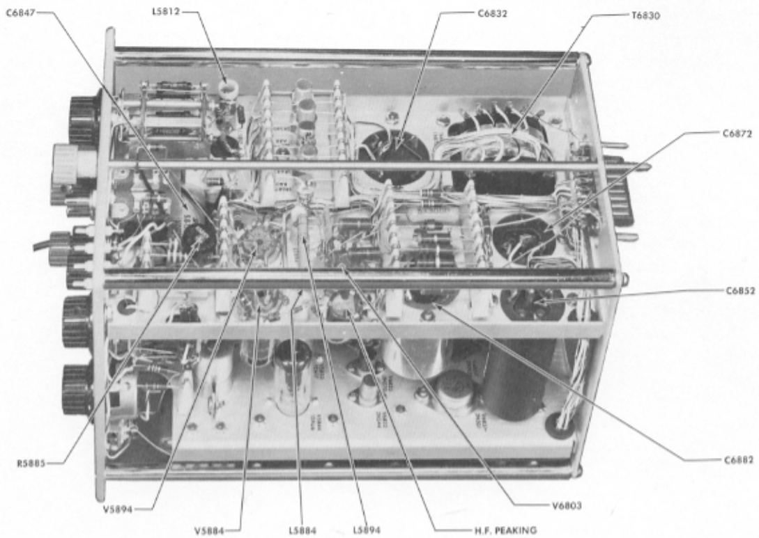
Fig. 5-8. Bottom and left side view of the Type R Unit.
