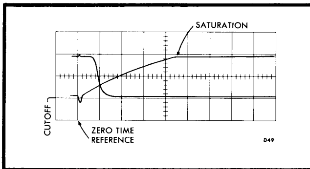
Fig. 2-9. Switching characteristics of a type 2N109 operating in the grounded-emitter configuration.
