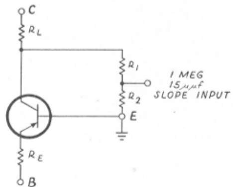
Fig. 2-13. Typical grounded-base transistor mounting board circuit.
