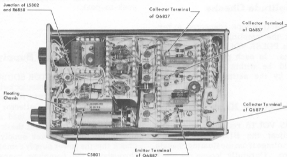
Fig. 5-2. Location of power supply test points.
