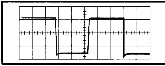
Fig. 5-3. Adjustment of the HF PEAKING control. The illustration above shows the typical waveform obtained with the correct setting of the HF PEAKING control.
