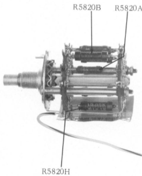
Type R BOTTOM VIEW SERIES RESISTOR A
