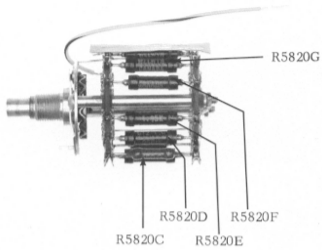
Type R TOP VIEW SERIES RESISTOR A
