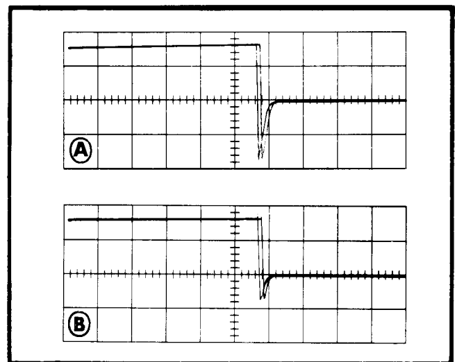
Fig. 5-5. Adjustment of L5812. Using a type 2N544 test transistor, L5812 is adjusted for a minimum of spiking on the falling portion of the pulse. A typical waveform obtained with the correct setting of L5812 is shown in illustration B. Waveform A results from a misadjustment of L5812.
